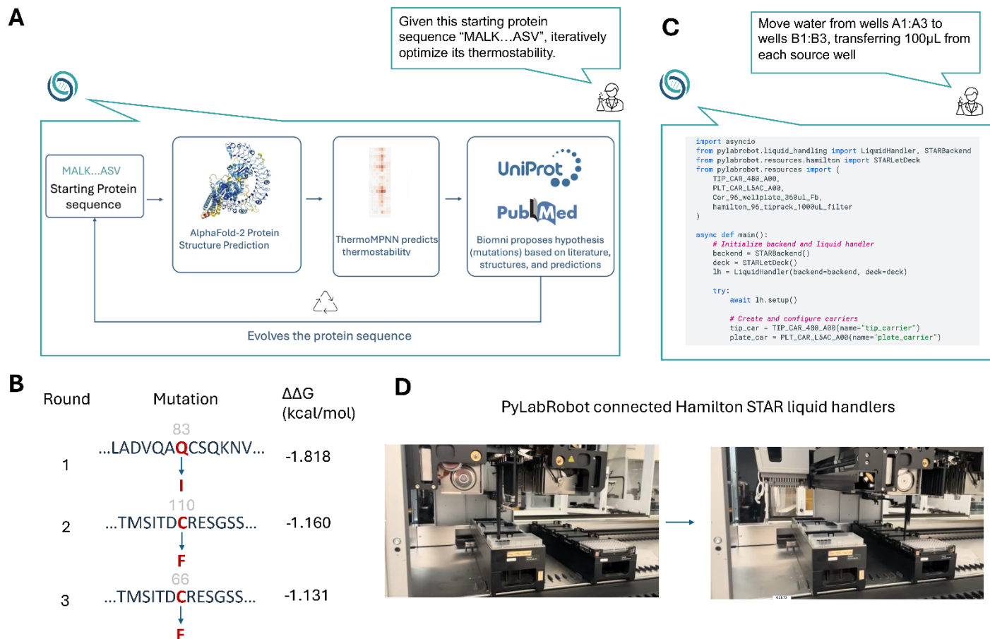
Fig. 5. AI-guided protein optimization and automated experimental execution. (A) Computational protein evolution pipeline. Biomni integrates structure prediction (AlphaFold-2), thermostability estimation (ThermoMPNN), and literature mining (UniProt/PubMed) to iteratively optimize a starting sequence ("MALK...ASV") for improved thermostability. (B) Example optimization trajectory. Over three iterative rounds, Biomni proposed stabilizing mutations (Q83I, C110F, C66F) yielding cumulative predicted \Delta\Delta G improvement of -4.108 kcal/mol, corresponding to enhanced core hydrophobicity and aromatic stabilization while maintaining 98% sequence identity. (C) AI-driven automation of experimental protocols. Biomni converts natural language descriptions of lab tasks (e.g., "Move water from wells A1-A3 to B1-B3, transferring 100 \mu L each") into fully executable PyLabRobot code. (D) The code was converted and validated on Hamilton STAR platforms for end-to-end digital-to-physical experiment execution.
